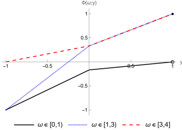
Fig. 4. Lehmann Accuracy Condition for F and G .
