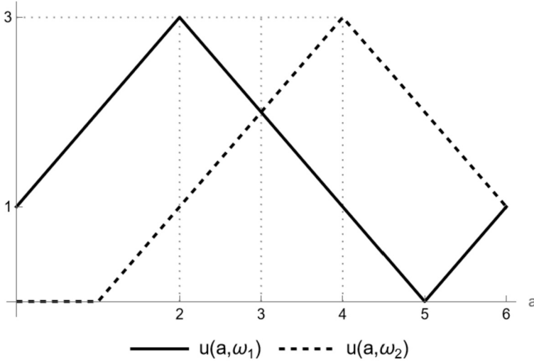
Fig. 5. Illustration of dominated decreasing decision rules, where the interval dominance property is violated.
