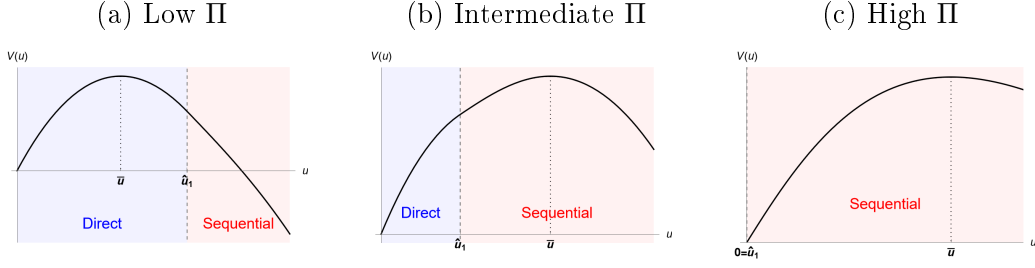
Figure 2: Value functions when there is no efficiency loss
