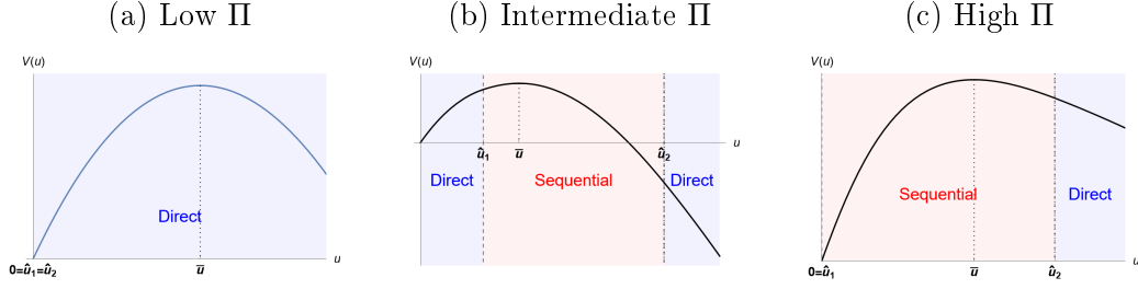
Figure 3: Value functions when the efficiency loss is small
