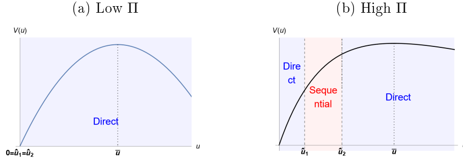
Figure 4: Value functions when the efficiency loss is large
